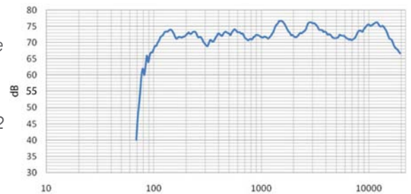
Response of a CEAD Adhesive ceiling tile speaker adhered to 1/2 inch (13mm) plasterboard
